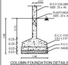
COLUMN FOUNDATION DETAILS
