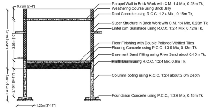
SECTIONAL VIEW ON A-A'
