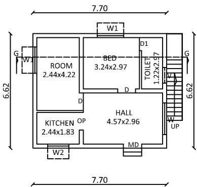
GROUND FLOOR PLAN (EXG)
