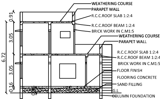
SECTION ON GG
