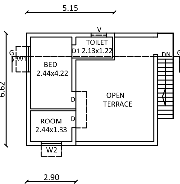
FIRST FLOOR PLAN (PRO)
