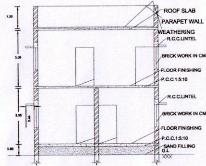
SECTION ON SS
