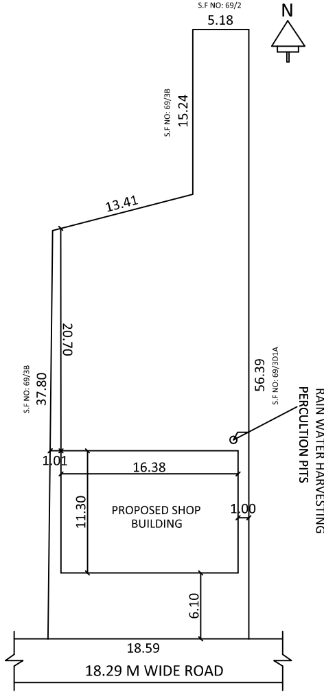
SITE PLAN
