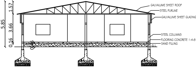
SECTION- SS
