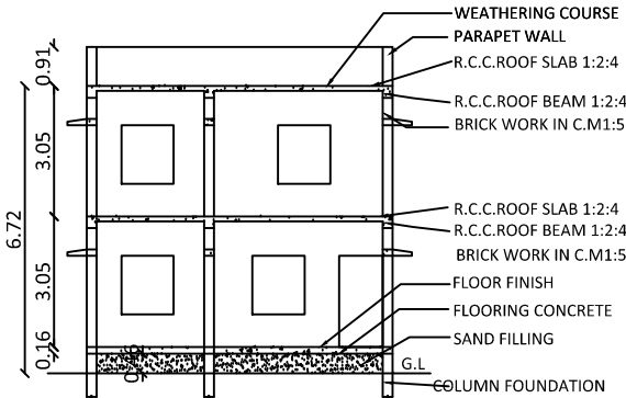
SECTION ON GG
