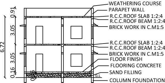
SECTION-SS
