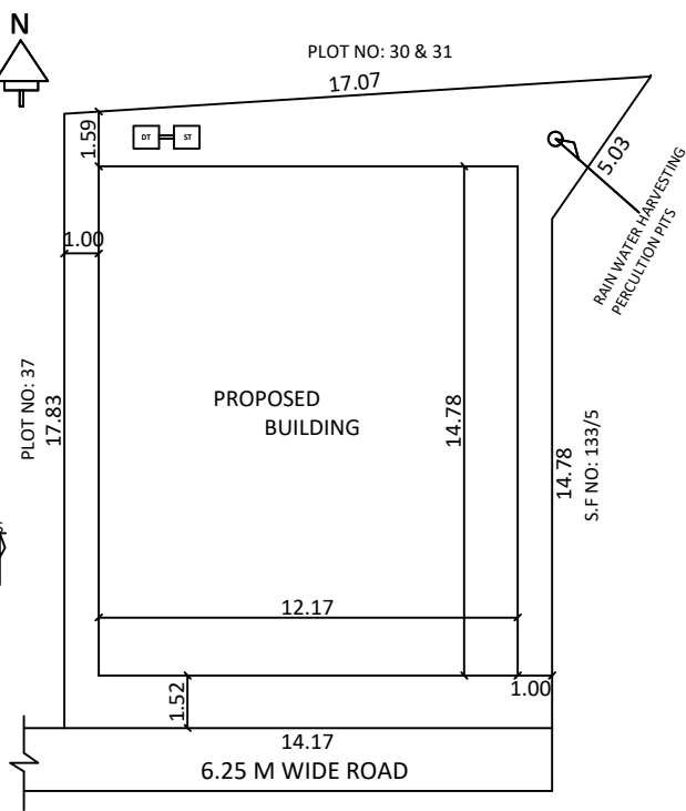
SITE PLAN
