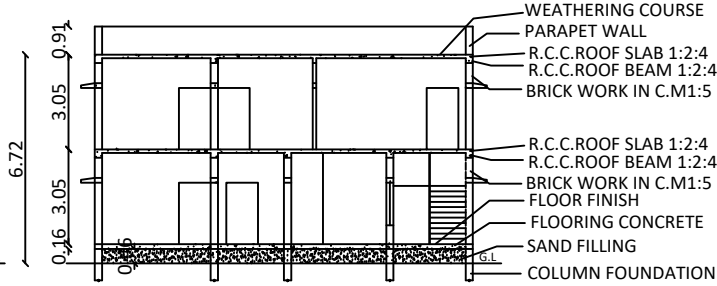
SECTION-SS
