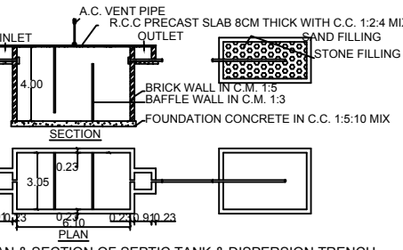
PLAN & SECTION OF SEPTIC TANK & DISPERSION TRENCH
