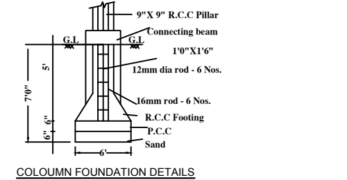
COLOUMN FOUNDATION DETAILS
