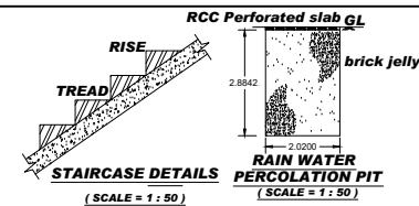
STAIRCASE DETAILS
