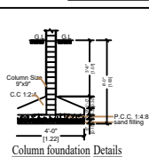
Column foundation Details
