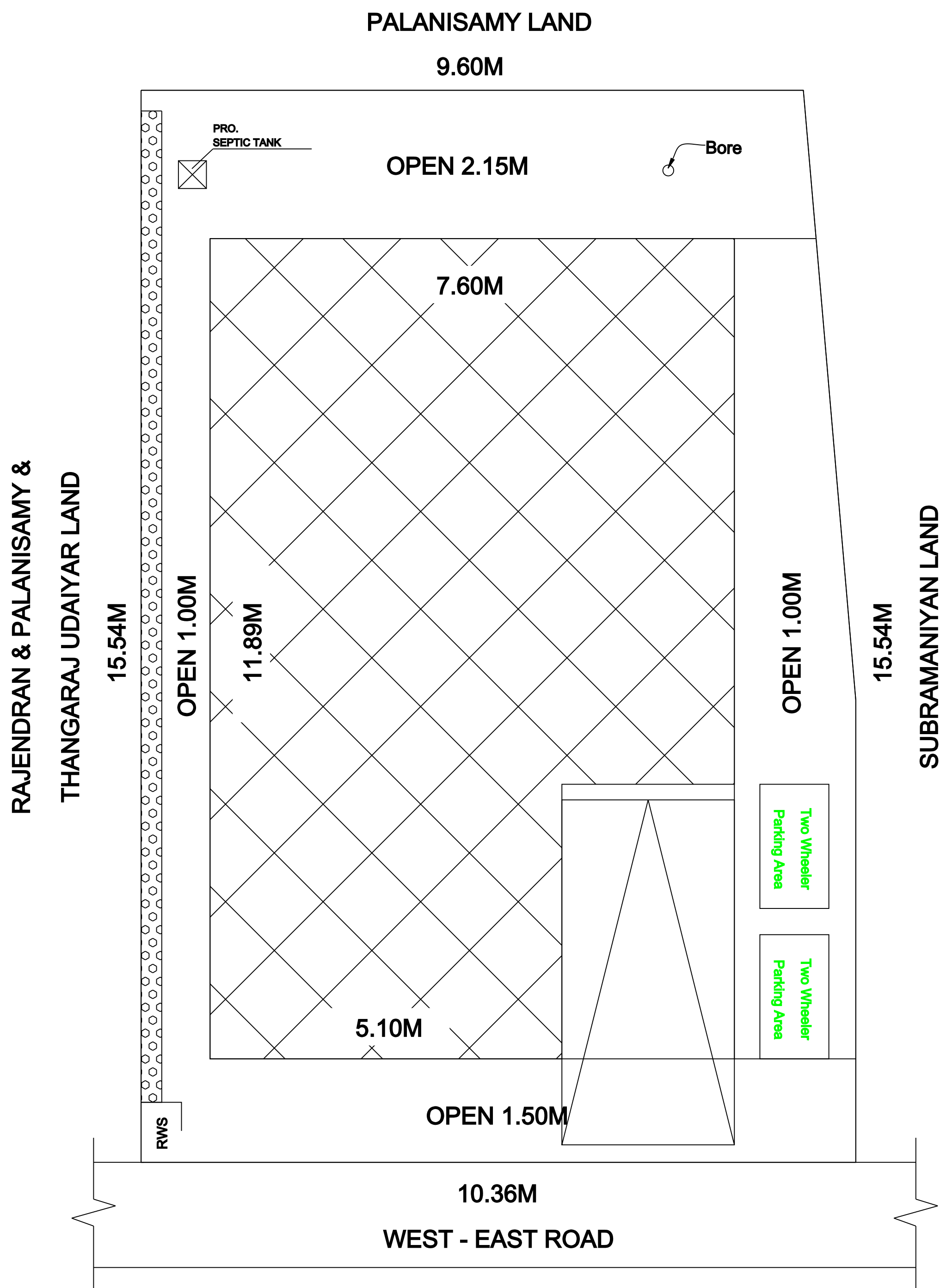
SITE PLAN
