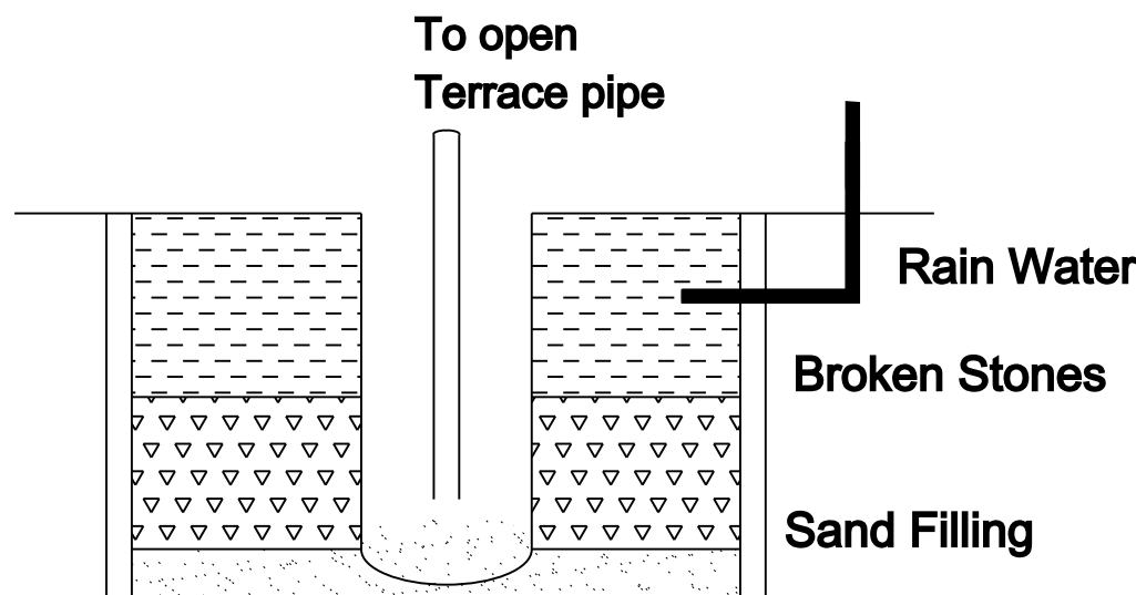
RAIN WATER COLLECTION CHAMBER
