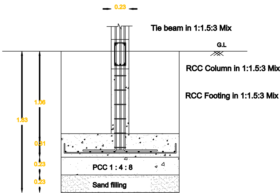
FOUNDATION DETAILS
