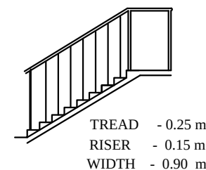
STAIRCASE DETAILS
