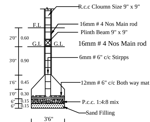
COLUMN DETIAL
