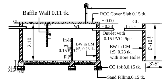
SECTION - SEPTIC TANK &amp; SOAK PIT
