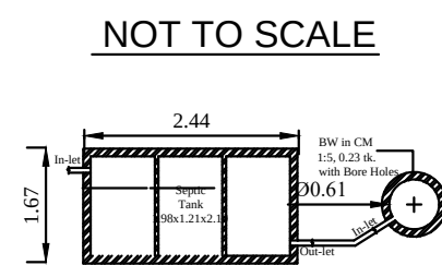
PLAN - SEPTIC TANK & SOAK PIT
