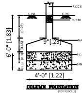
COLUMN FOUNDATION (NOT TO SCALE)
