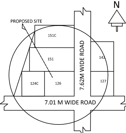
LOCATION PLAN
