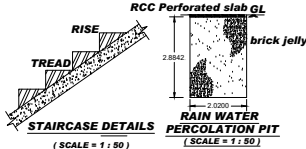
STAIRCASE DETAILS
