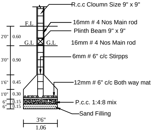
COLUMN DETIAL
