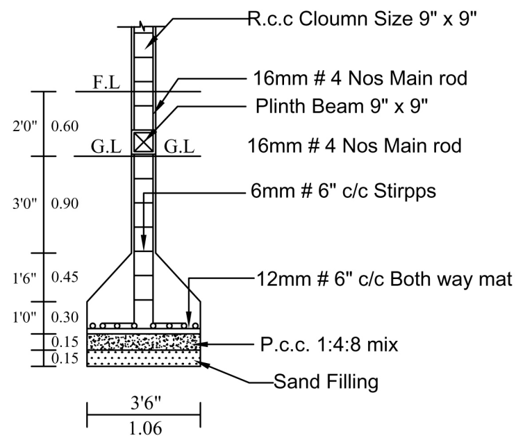
COLUMN DETIAL
