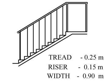
STAIRCASE DETAILS
