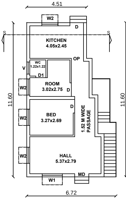
GROUND FLOOR PLAN (EXG)
