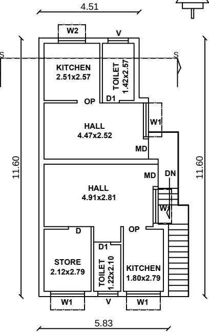
FIRST FLOOR PLAN (PRO)
