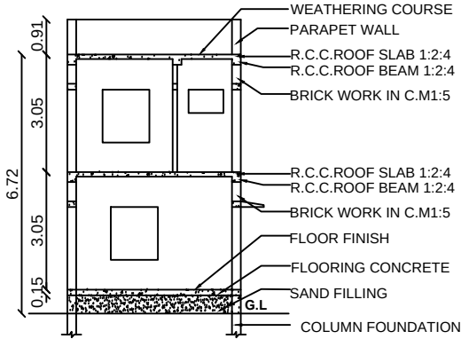
SECTION ON SS
