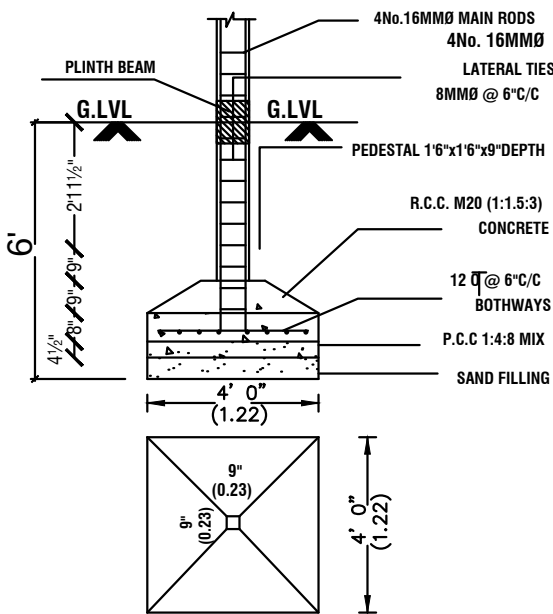
FOUNDATION DETAILS
