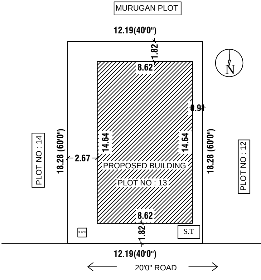
SITE PLAN
