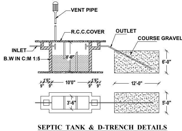
SEPTIC TANK & D-TRENCH DETAILS (NOT TO SCALE)
