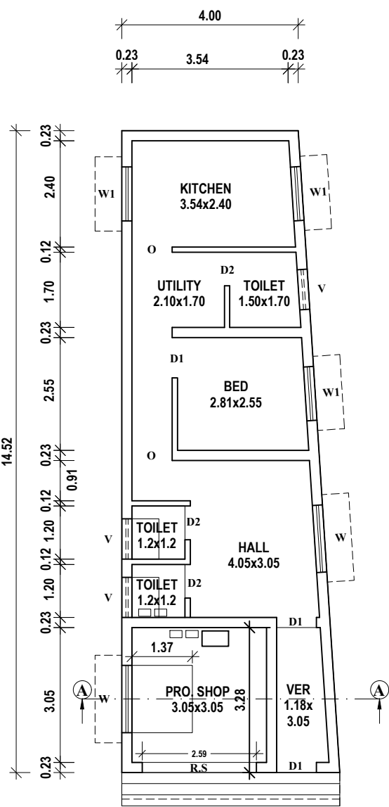
EXG & PRO. GROUND FLOOR PLAN
