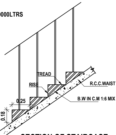
SECTION OF STAIRCASE
