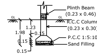
FOUNDATION DETAILS
