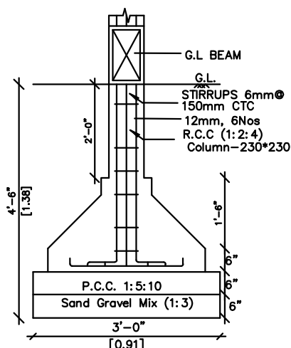
R.C.C. COLUMN FOOTING DETAILS SCALE : 1:25
