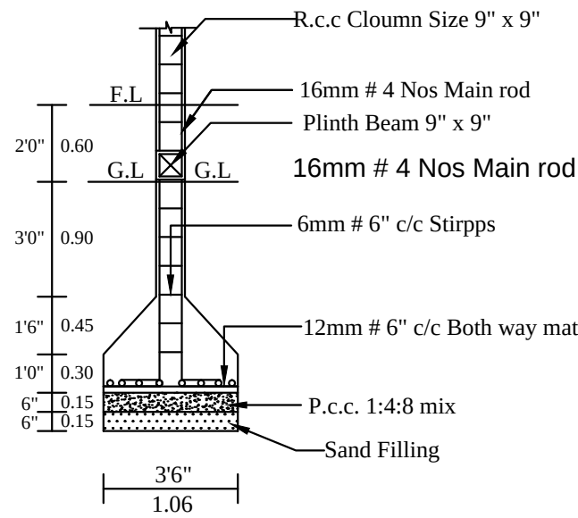
COLUMN DETIAL
