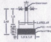
FOUNDATION DETAILS (Scale = 1:50)
