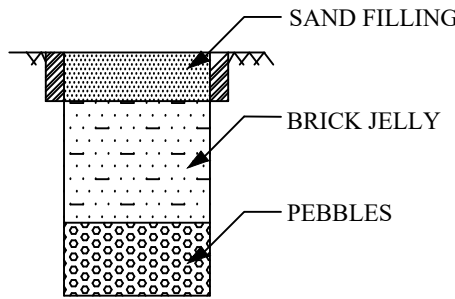
RWH SYSTEM
