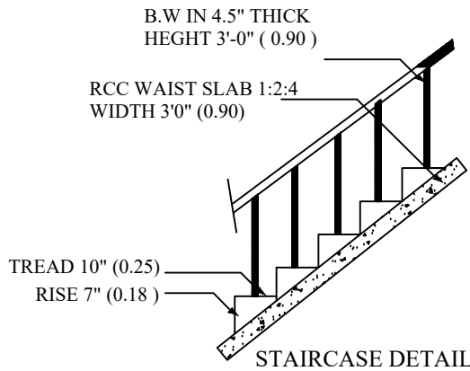
STAIRCASE DETAIL ( SCALE 1:50 )
