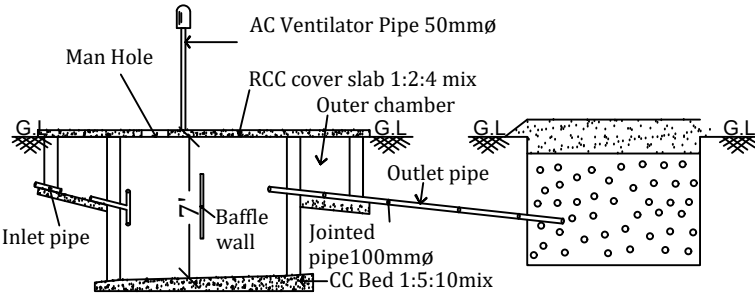
SECTION FOR SEPTIC TANK AND D.T
