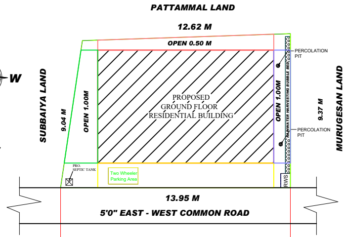
SITE PLAN (SCALE 1:1)
