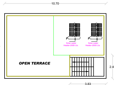
OPEN TERRACE PLAN
