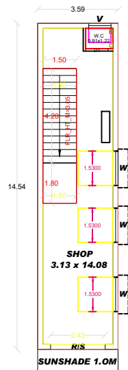
GROUND FLOOR PLAN
