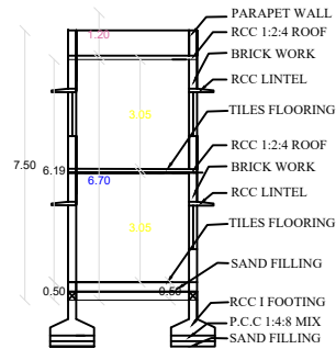
SECTION ON AB
