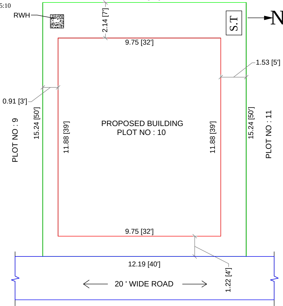
SITE PLAN
