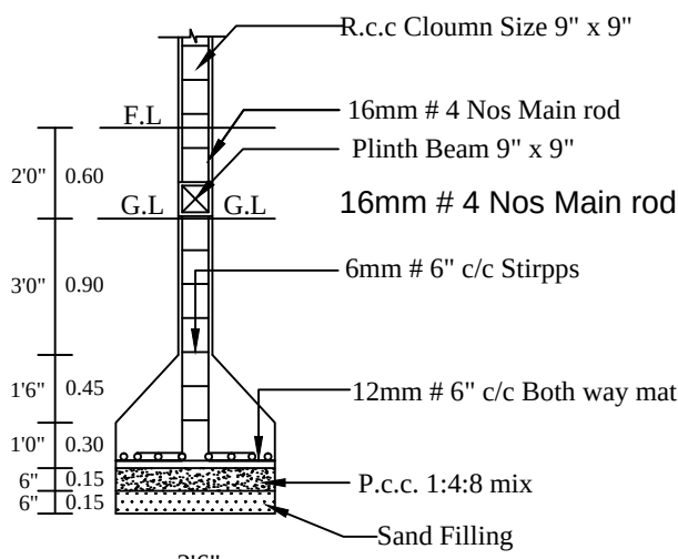
COLUMN DETIAL
