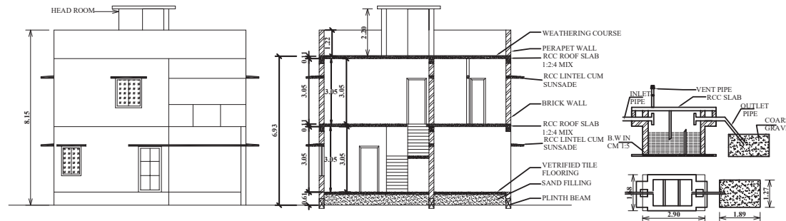
SEPTIC TANK & D-TRENCH DETAILS (NOT TO SCALE)
