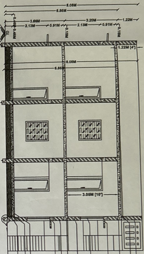
SECTION ON A-B
