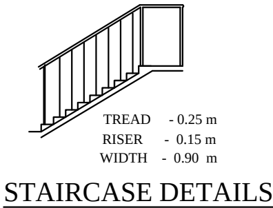
STAIRCASE DETAILS
