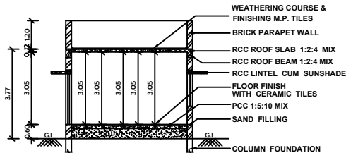
SECTION ON A-A
