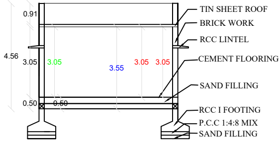
SECTION ON AB RATHINAM LAND 7.92 M
