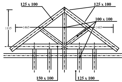
TRUSS DETAILS (IN MM)
