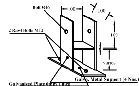
UPPER BOLTS DETAILS (IN MM)
