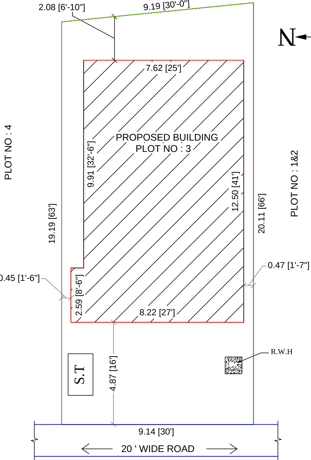
SITE PLAN
