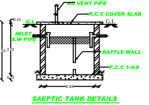
SAEPTIC TANK DETAILS
