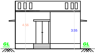
FRONT ELEVATION
