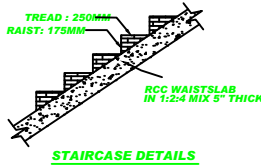
STAIRCASE DETAILS
