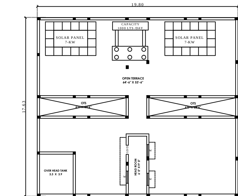
PROPOSED OPEN TOP TERRACE PLAN
