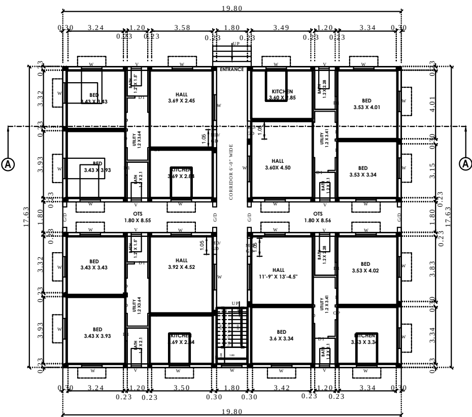
TYPICAL_FLOOR_PLAN=0.1 PROPOSED GROUND FLOOR PLAN
