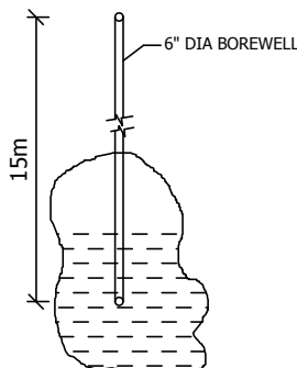
BORE WELL DETAIL (NOT TO SCALE)
