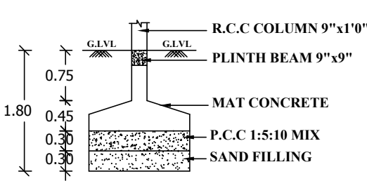
COLUMN FOUNDATION (NOT TO SCALE)
