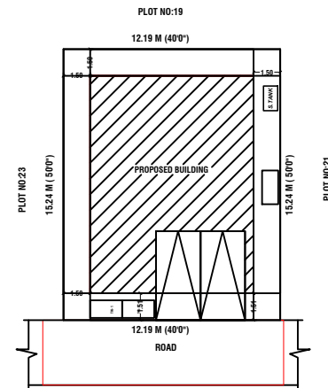
SRI VENKATESA NAGAR SITE SITE PLAN (SCALE: 1:100)
