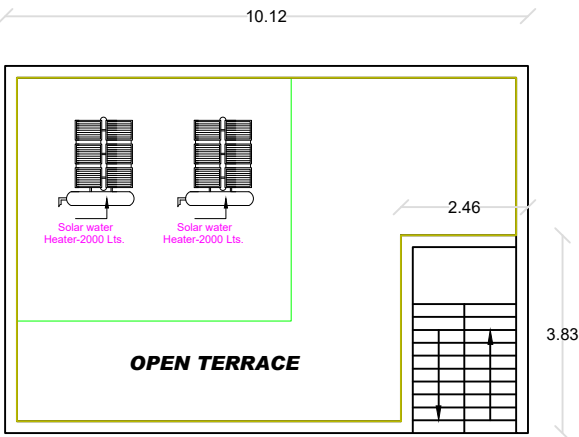
OPEN TERRACE PLAN
