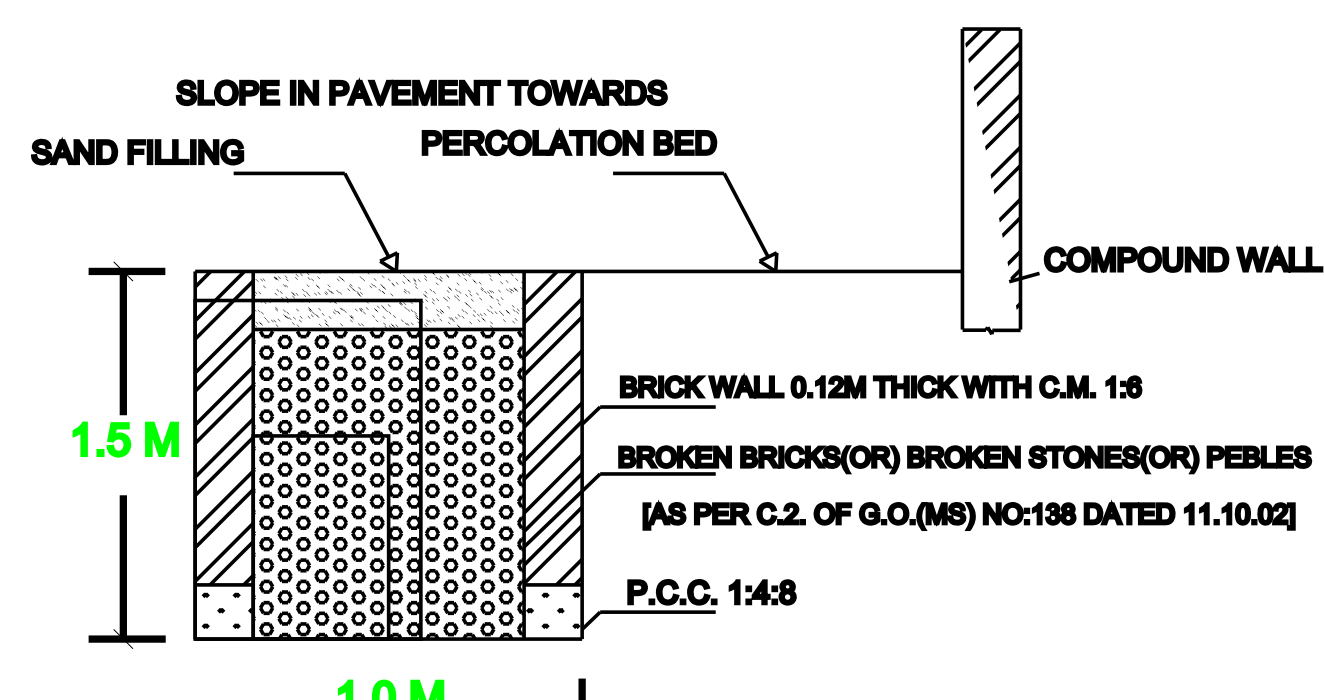
SECTION OF RAIN WATER PERCOLATION BED
