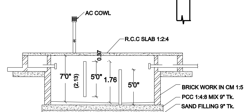
SECTION
