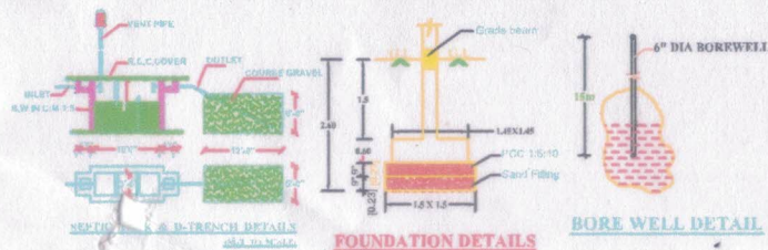
FOUNDATION DETAILS
