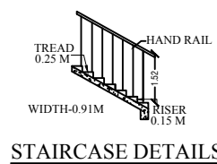
STAIRCASE DETAILS
