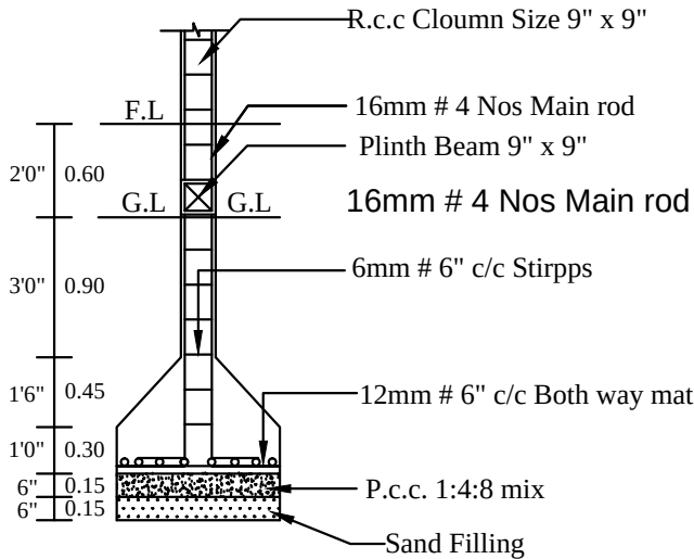
COLUMN DETIAL
