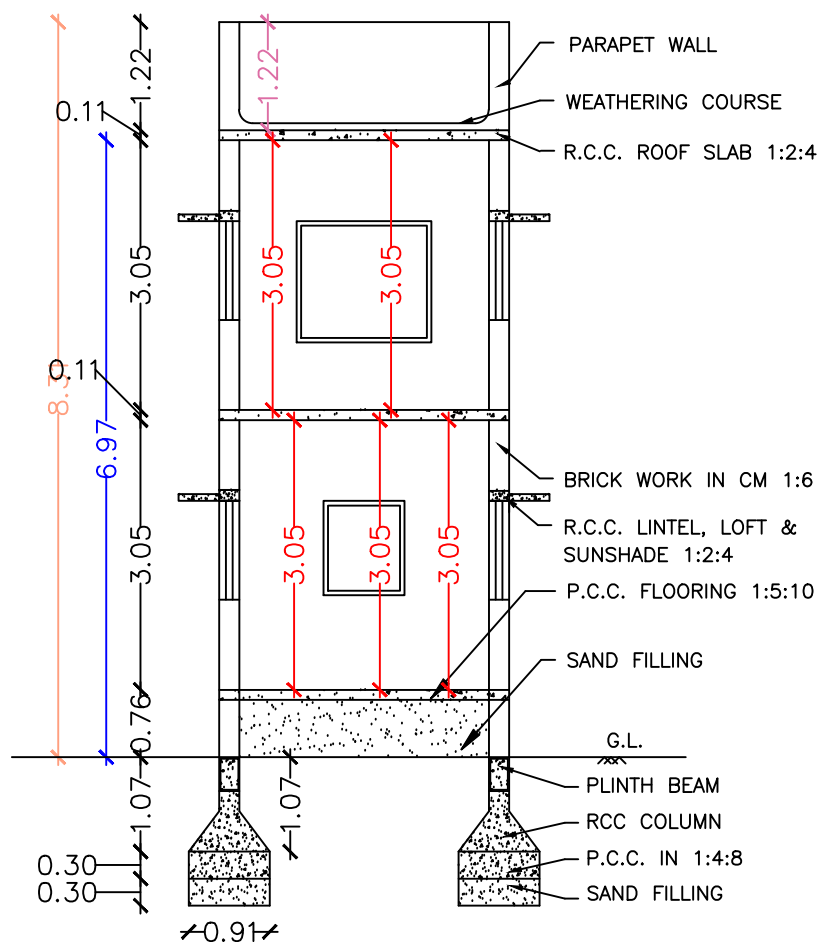
SECTION AA
