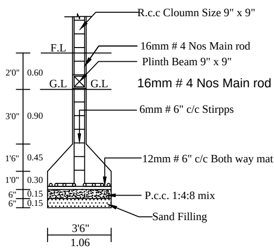
COLUMN DETIAL
