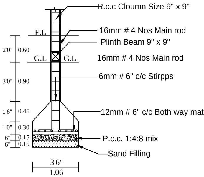
COLUMN DETIAL
