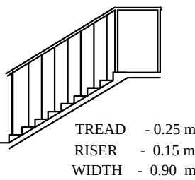
STAIRCASE DETAILS
