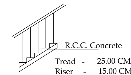
Staircase details
