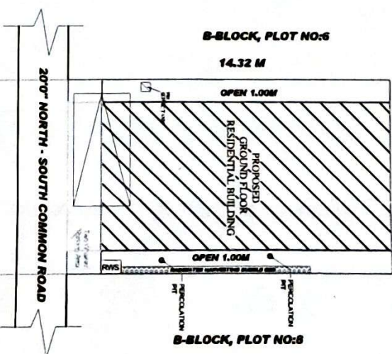
SITE PLAN (SCALE 1:1)
