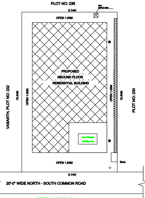
SITE PLAN (SCALE 1:1)
