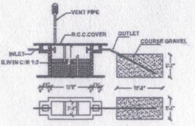
SEPTIC TANK & D-TRENCH DETAILS (NOT TO SCALE)
