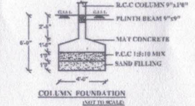
COLUMN FOUNDATION (NOT TO SCALE)
